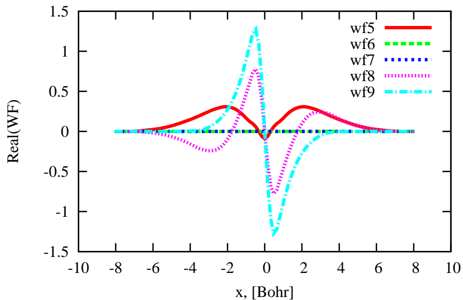
Graphene WaveFunctions@Gamma, slice zkz
