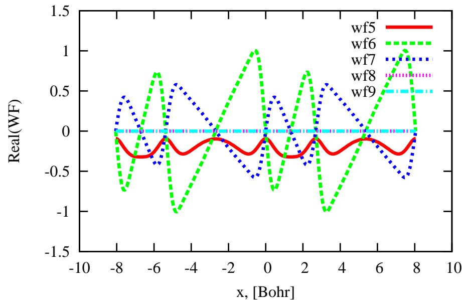
Graphene WaveFunctions@Gamma, slice kmkgkmkgk
