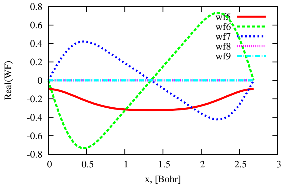
Graphene WaveFunctions@Gamma, slice kmk
