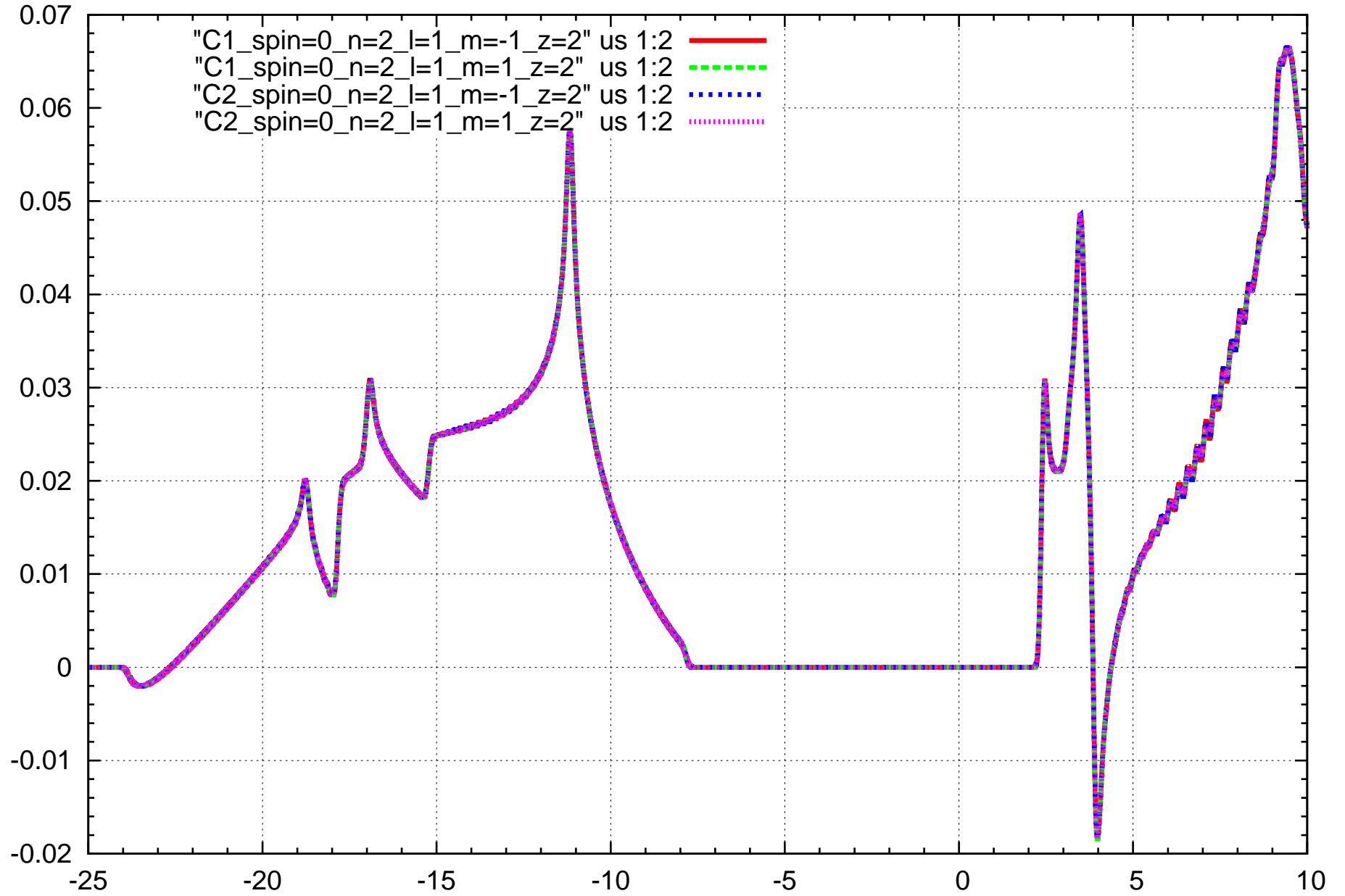
Graphene PDOS
