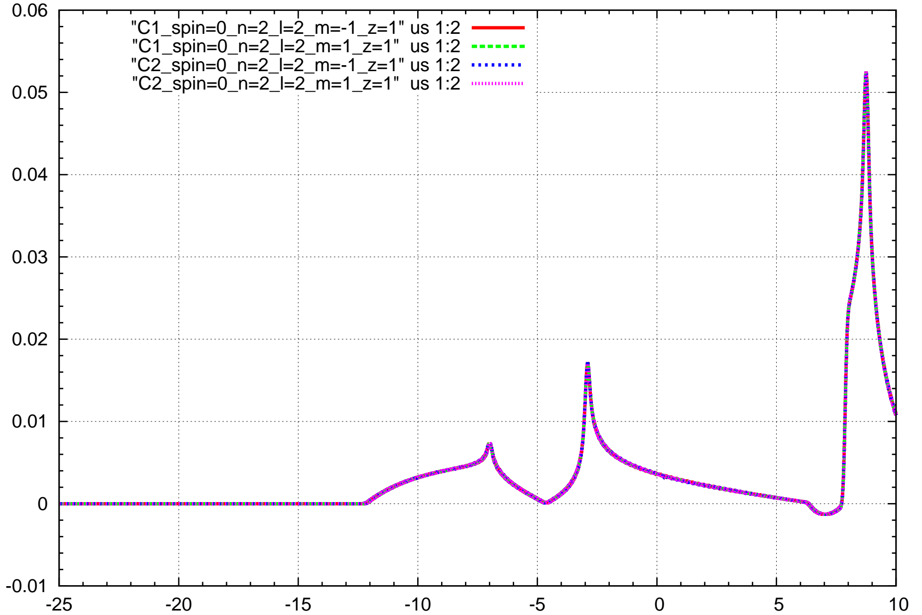
Graphene PDOS
