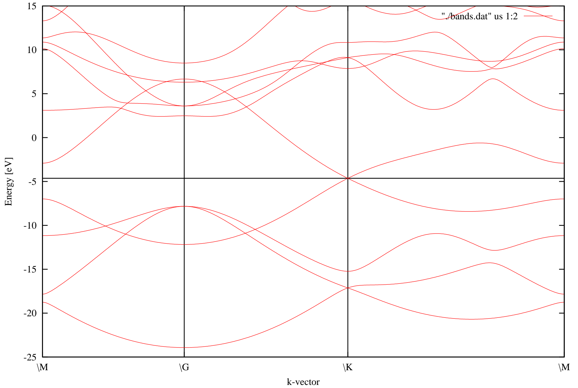
Graphene electronic bands
