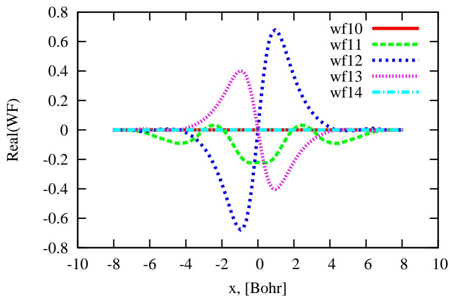
Graphene WaveFunctions@Gamma, slice zmz
