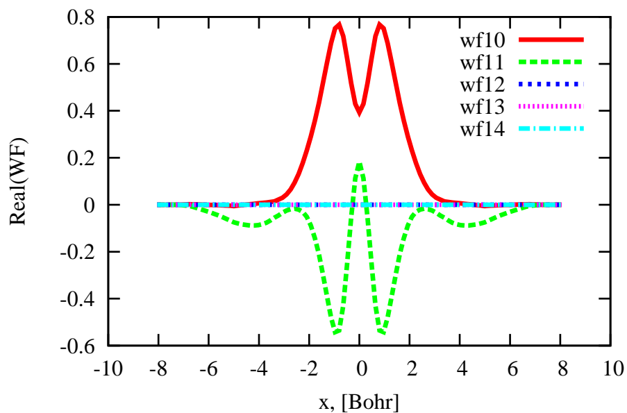
Graphene WaveFunctions@Gamma, slice zkz
