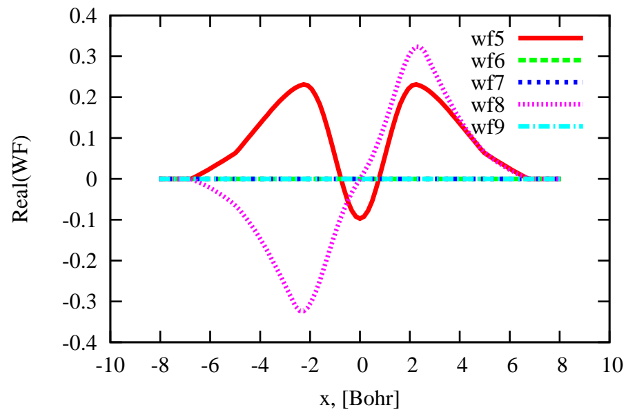
Graphene WaveFunctions@Gamma, slice zgz
