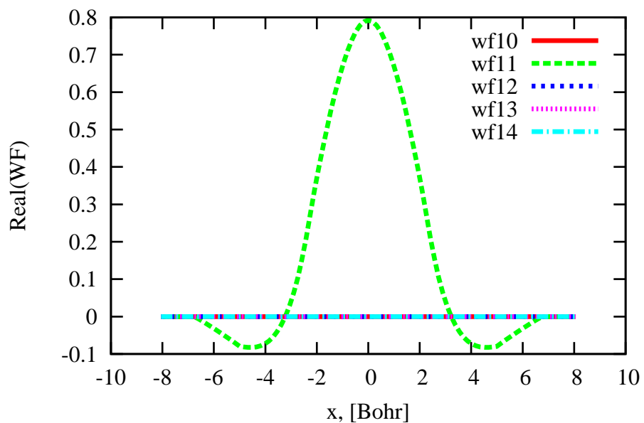
Graphene WaveFunctions@Gamma, slice zgz
