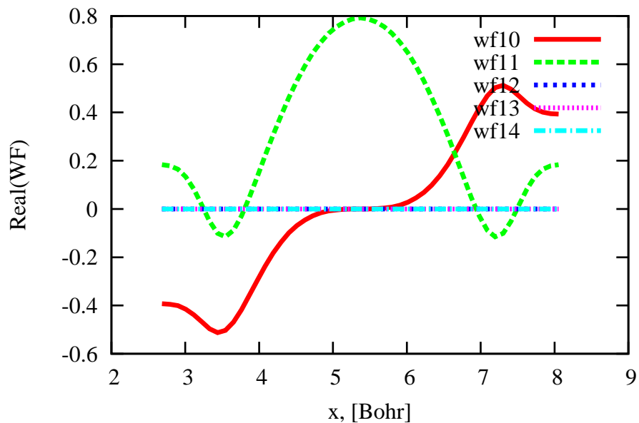
Graphene WaveFunctions@Gamma, slice kgk
