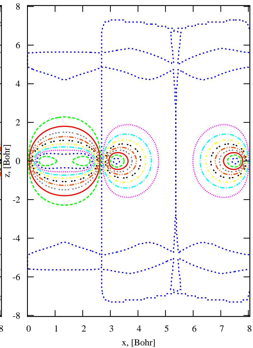
Graphene 2D WF4 @Gamma, slice xkz
