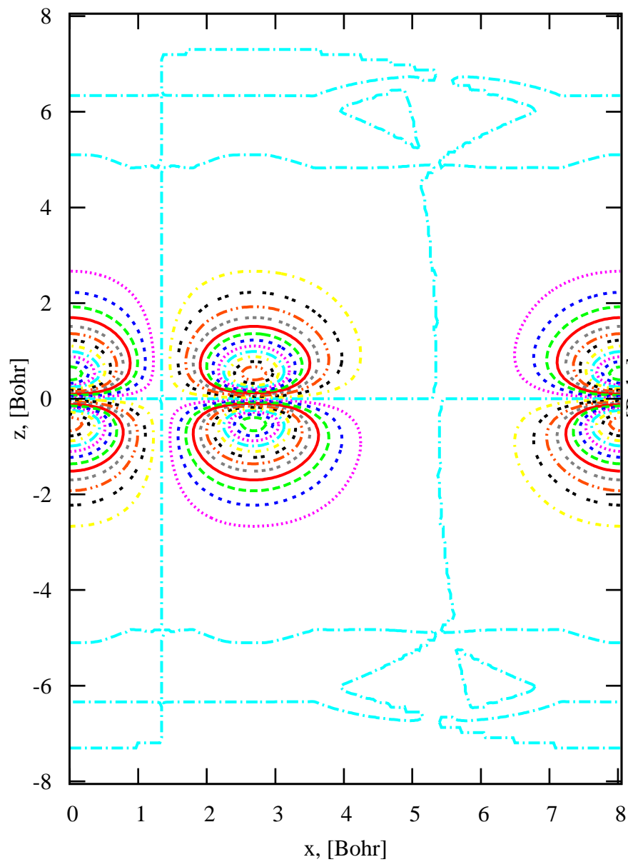
Graphene 2D WF9 @Gamma, slice xkz
