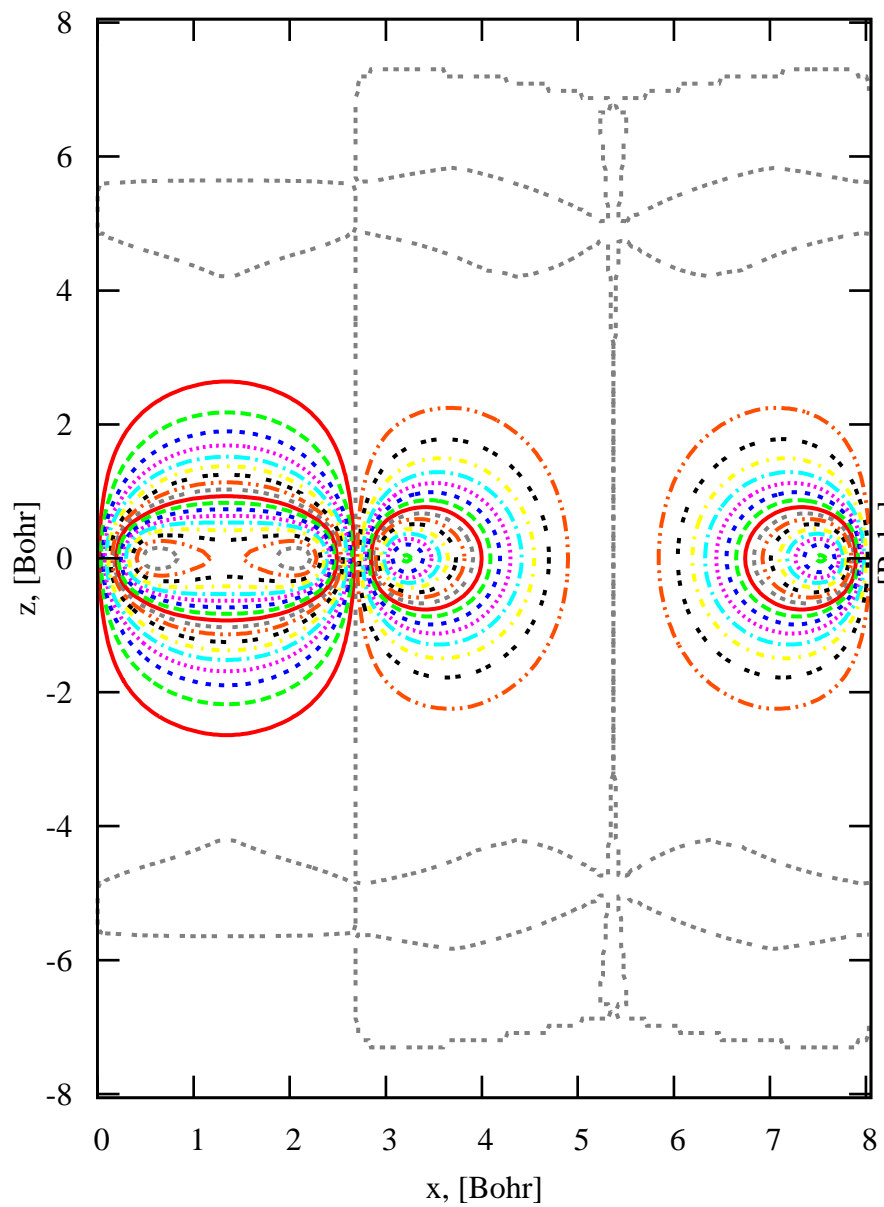
Graphene 2D WF3 @Gamma, slice xkz
