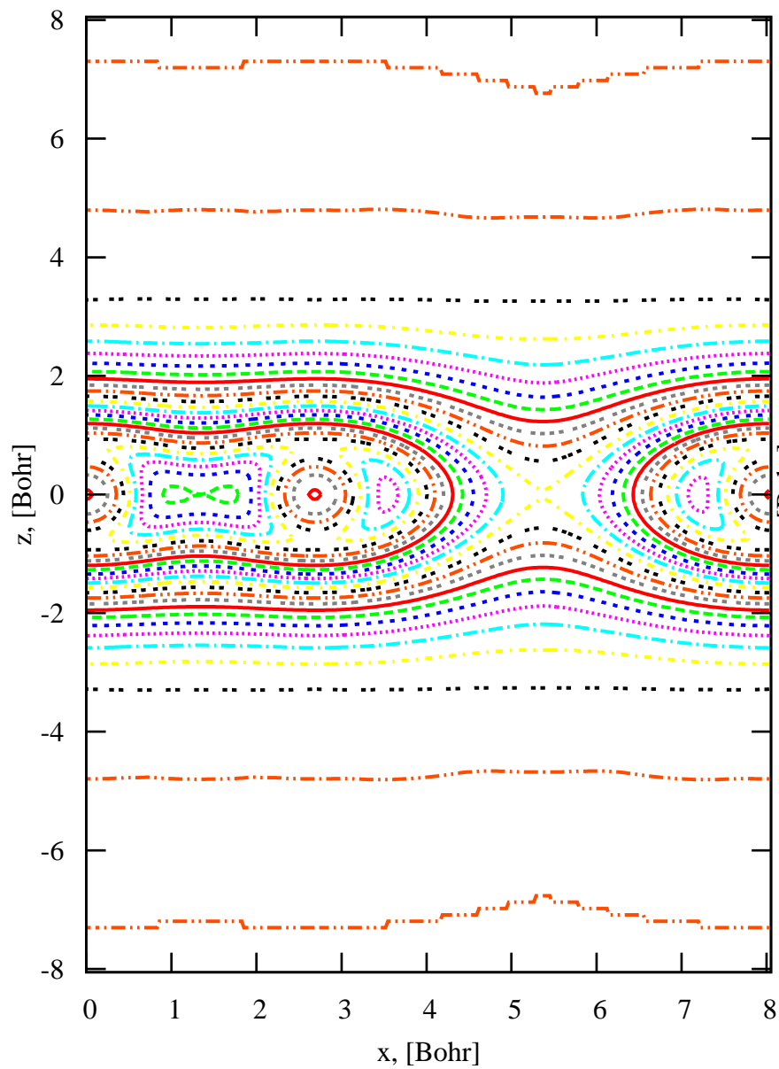
Graphene 2D WF1 @Gamma, slice xkz
