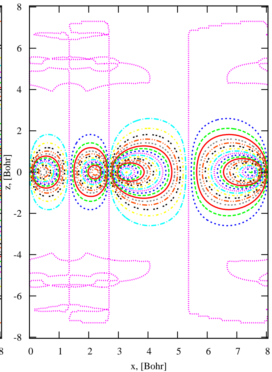
Graphene 2D WF6 @Gamma, slice xkz
