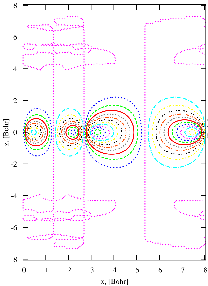
Graphene 2D WF7 @Gamma, slice xkz
