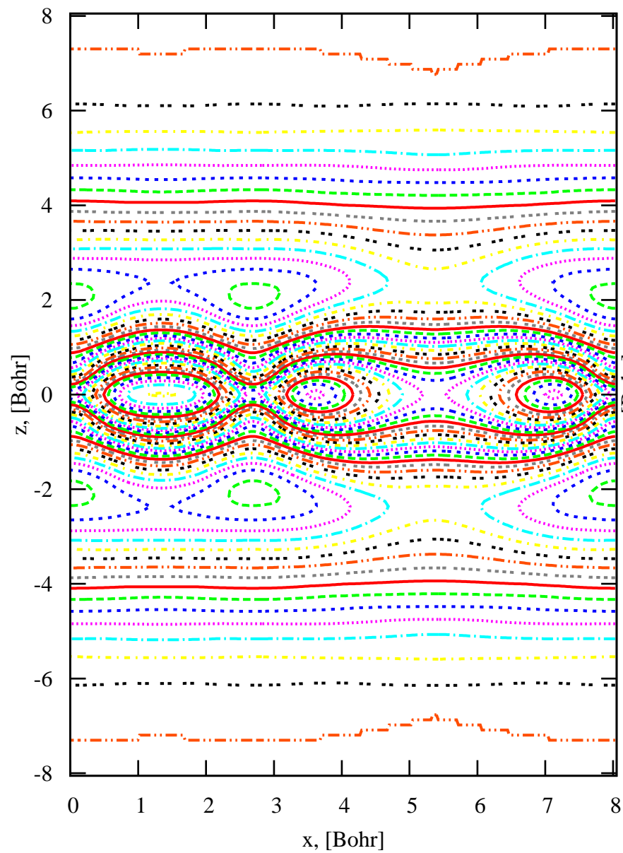
Graphene 2D WF5 @Gamma, slice xkz
