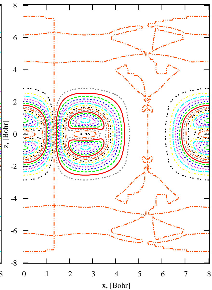
Graphene 2D WF10 @Gamma, slice xkz
