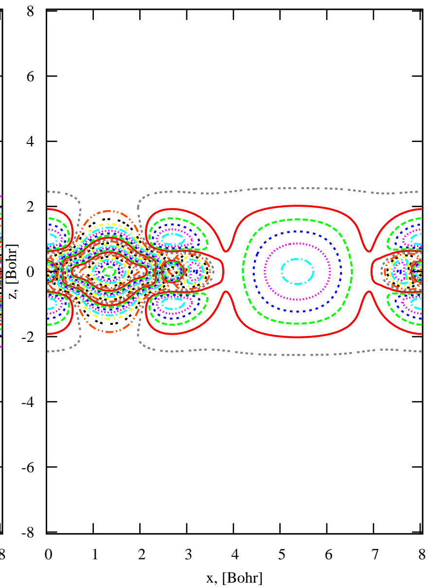
Graphene 2D charge DEL @Gamma, slice xkz
