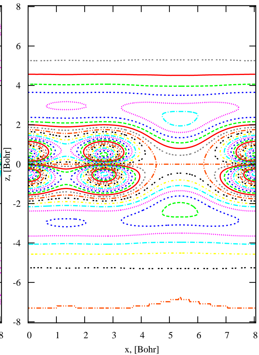
Graphene 2D WF8 @Gamma, slice xkz
