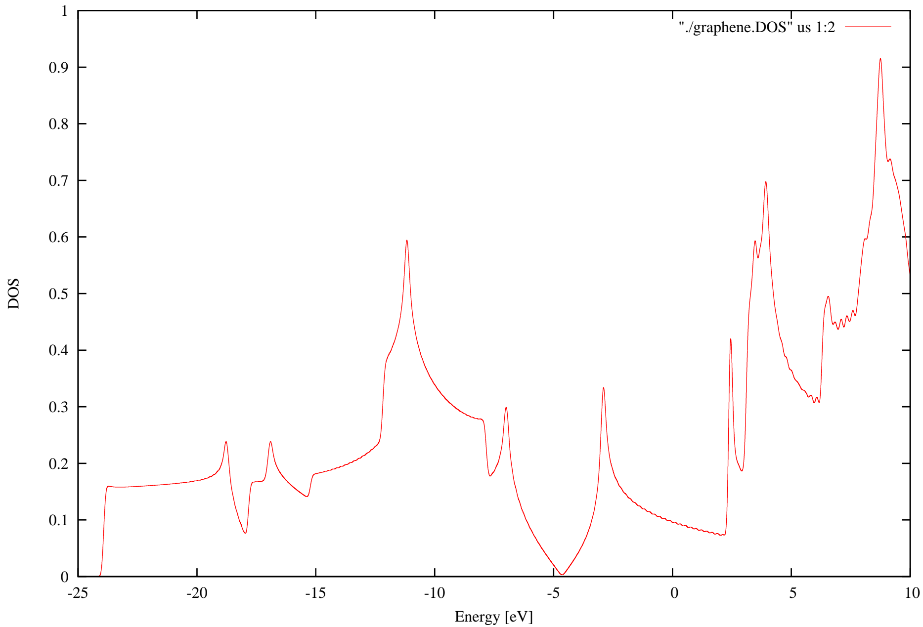
Graphene DOS
