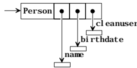
Figure 3.9: Pictorial representation of a record Person.
